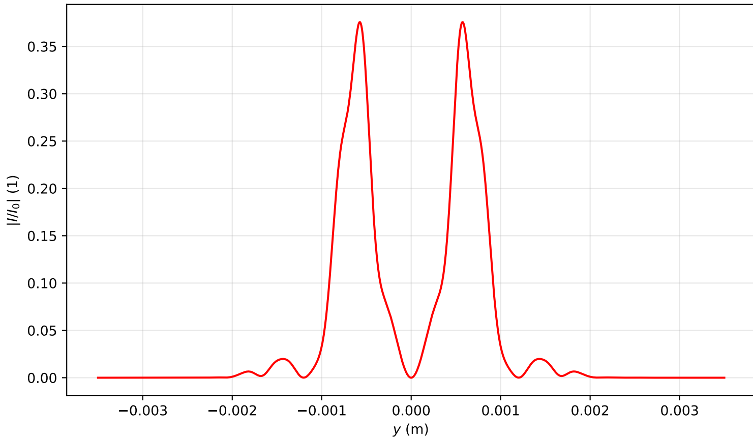
Intensity profile I(x=0, y, z=1.353)/I_0 , P_{in}=6.0P_{cr} , artificial time
